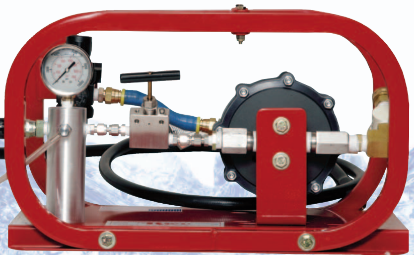
HP-10 • 10,000 PSI
