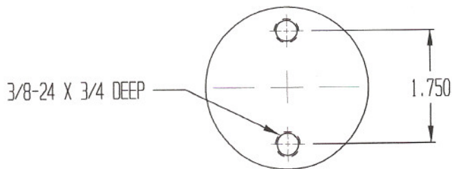
MOUNTING DIMENSIONS
